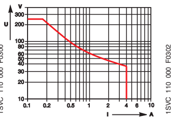
Resistive DC load
