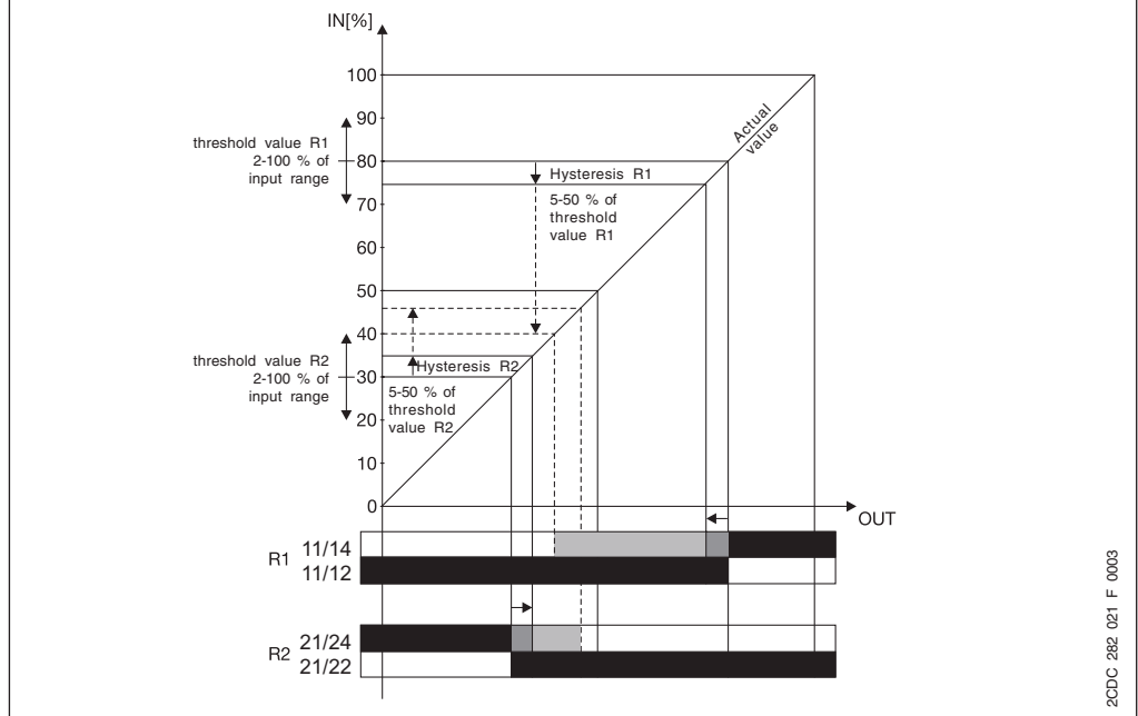
Switching points of the output relay depending on the input range, configuration open-circuit principle
